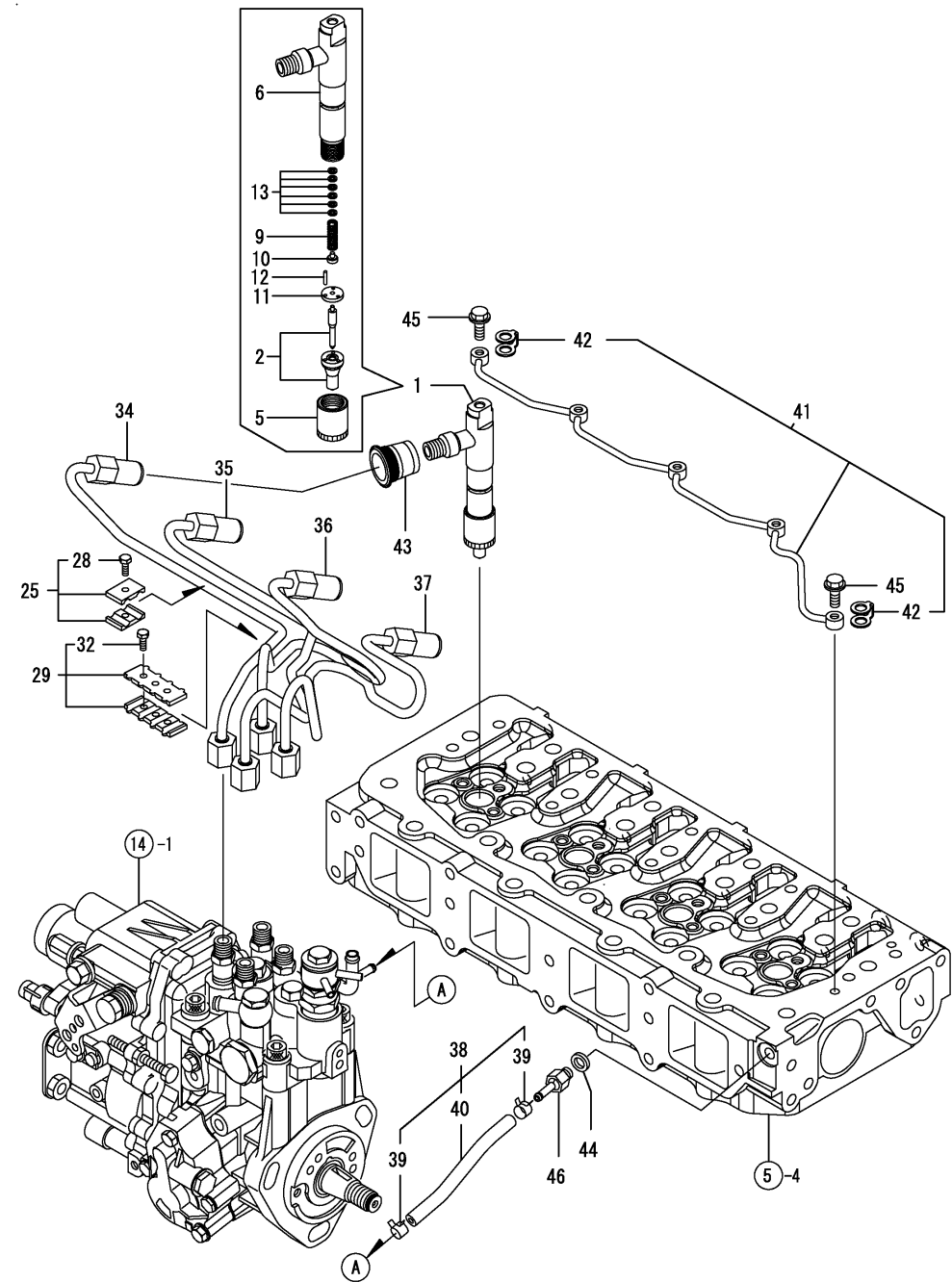
Fig.16. FUEL INJECTION VALVE
