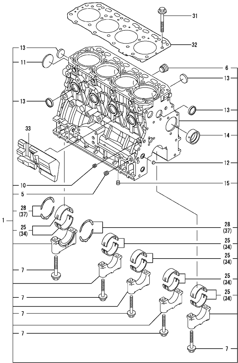
Fig.1. CYLINDER BLOCK
