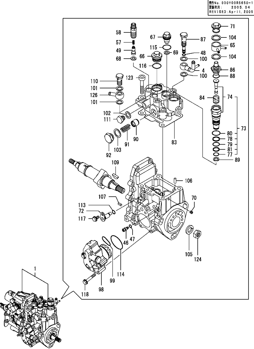
Fig.25. FUEL INJECTION PUMP(INNER PARTS)
